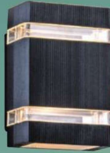
SH-24543 3250 W110mm H170mm D100mm 附LED 6Wx1 黃光 鋼材烤漆
